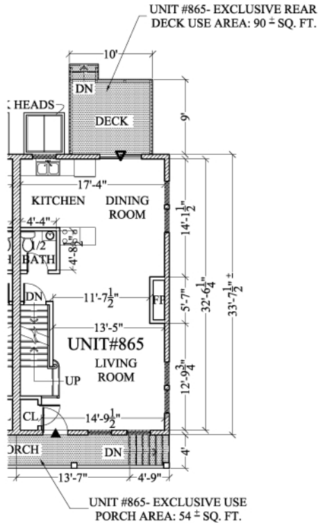
FIRST FLOOR PLAN UNIT #865 LIVING AREA 563 SQ. FT. ±
